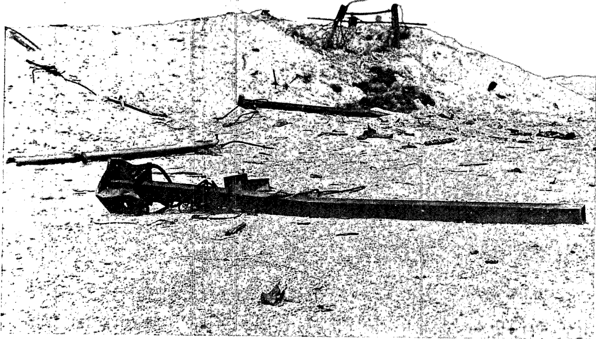
Fig. 8—Post-Quay event damage, horizontal view of tower-base area.
